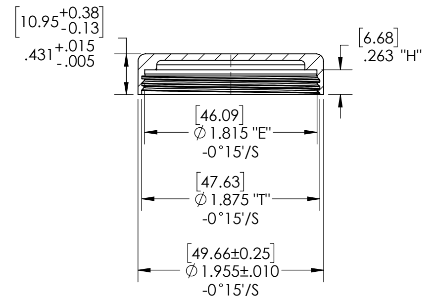
SECTION C-C
